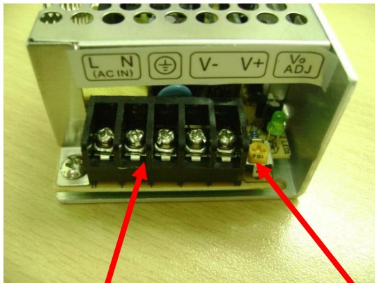
DC 12V Output to Controller
